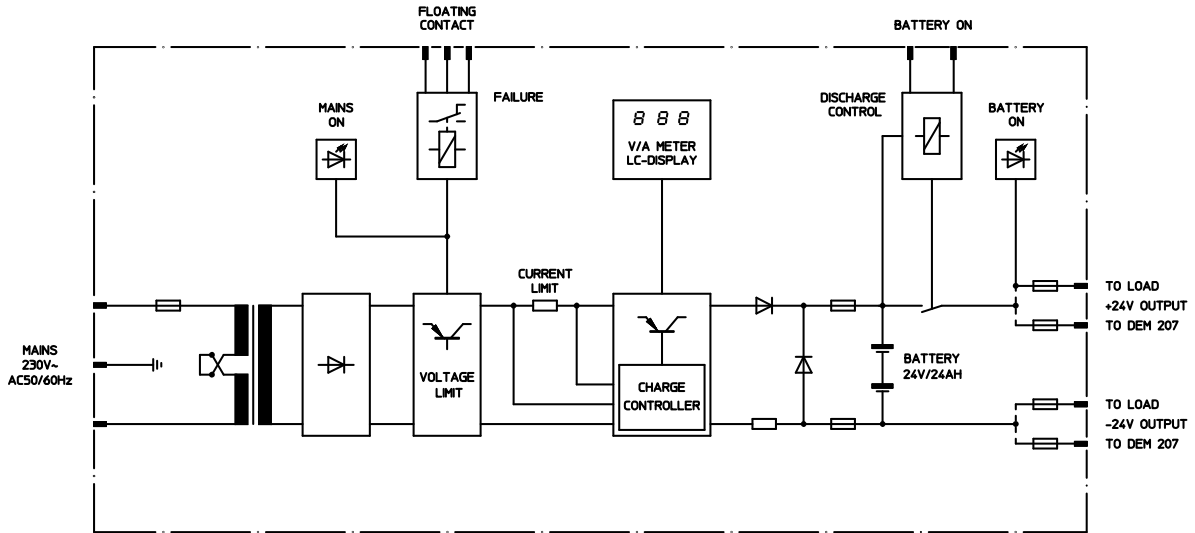
Block-Diagram 347 790
